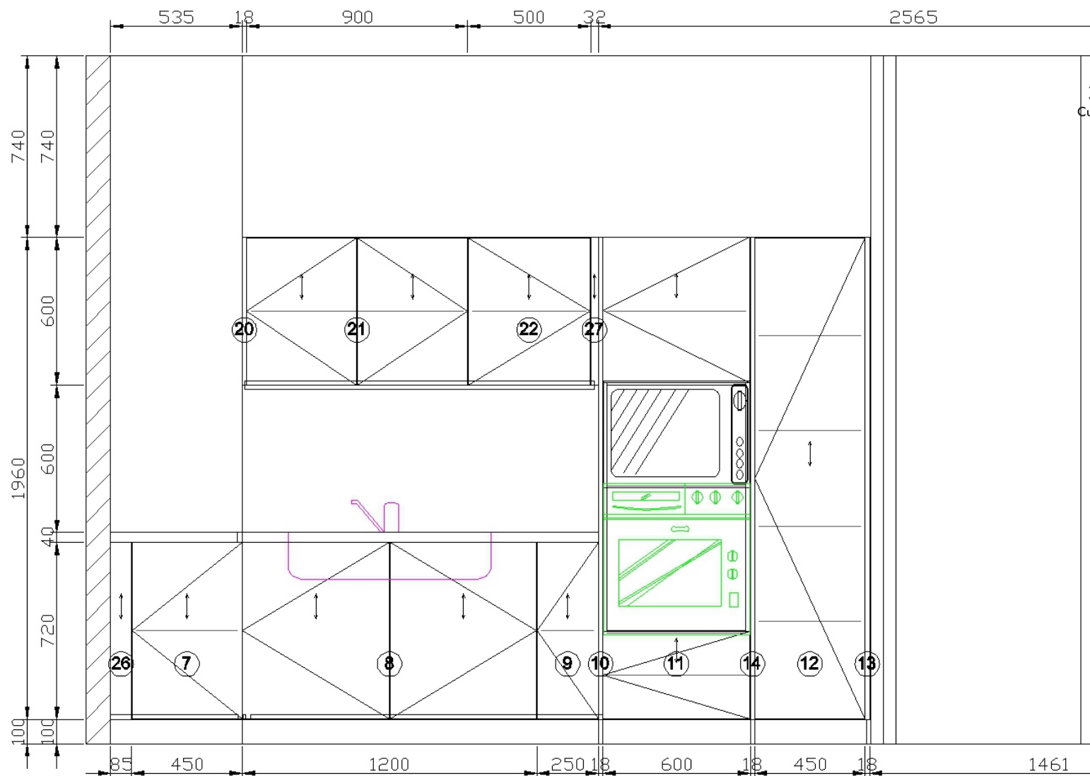
A View elevation drawing
